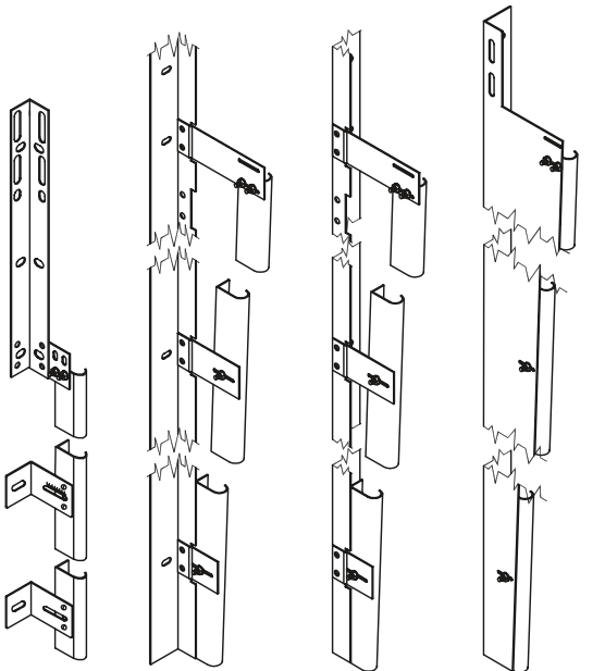
2" BRACKET MOUNT
